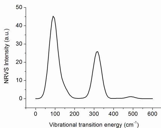
Figure 5.23: Theoretical IR spectrum with the shapes of vibrations dominating the IR intensity and NRVS scattering
